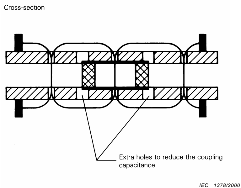
Figure A.2c – Details of transformer core construction
